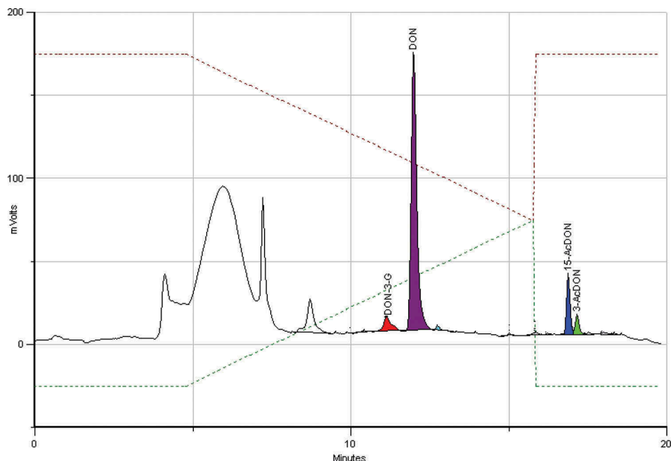
Figure 6. (colour online) IAC-HPLC-PCD-FLD chromatogram of a maize sample contaminated with the following concentrations: DON – 131 \mu\text{g kg}^{-1} / DON-3-G – 17 \mu\text{g kg}^{-1} / 15-AcDON – 23 \mu\text{g kg}^{-1} and 3-AcDON – 9.8 \mu\text{g kg}^{-1} .
