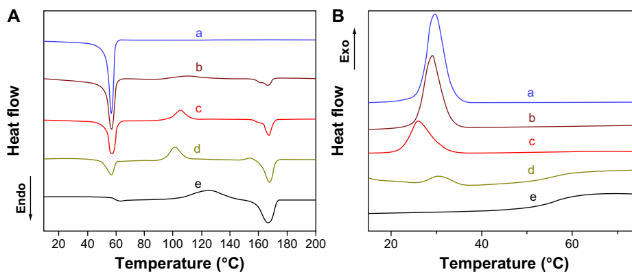
Figure 4 Differential scanning calorimetry curves of poly(lactide)/poly( \epsilon -caprolactone)-poly(ethylene glycol)-poly( \epsilon -caprolactone) (PCEC) hybrid fibrous scaffolds with 100 wt% (a), 75 wt% (b), 50 wt% (c), 25 wt% (d), and 0 wt% (e) PCEC concentrations.
