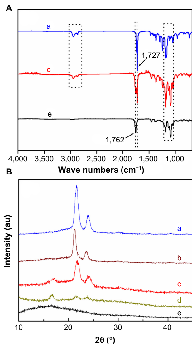
Figure 3 Fourier transform infrared spectra (A) and X-ray diffraction (B) patterns of polylactide/poly( \epsilon -caprolactone)-poly(ethylene glycol)-poly( \epsilon -caprolactone) (PCEC) nanofibrous membrane with 100 wt% (a), 75 wt% (b), 50 wt% (c), 25 wt% (d), and 0 wt% (e) PCEC concentrations.
