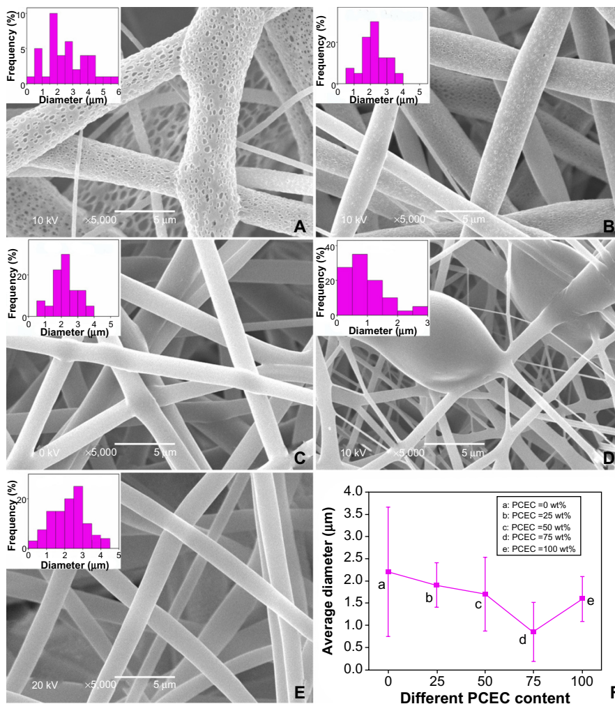
Figure 6 Scanning electron microscope photographs and the diameter distribution of the poly(lactide)/poly( \epsilon -caprolactone)-poly(ethylene glycol)-poly( \epsilon -caprolactone) (PCEC) hybrid fibers containing (A) 0, (B) 25, (C) 50, (D) 75, and (E) 100 wt% of PCEC.
