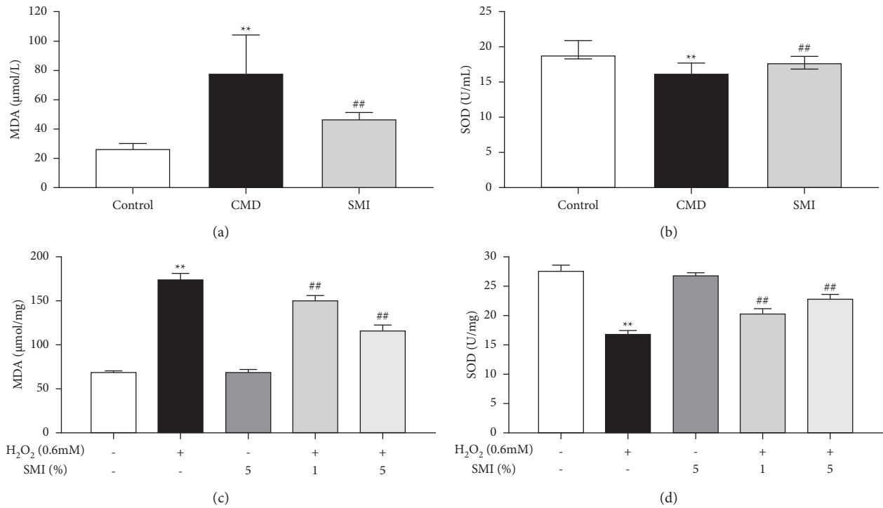
FIGURE 7: Effects of SMI on MDA (a) and SOD (b) in serum of CMD rats. Effects of SMI on MDA (c) and SOD (d) in HUVECs. Data are expressed as mean ± SD (n = 5). ** p < 0.01 vs. control group; ## p < 0.01 vs. CMD group.
