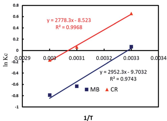
Fig. 10 Van't Hoff plot of adsorption for CR and MB adsorption onto Al 2 O 3 /GO/HNT nanocomposite.
