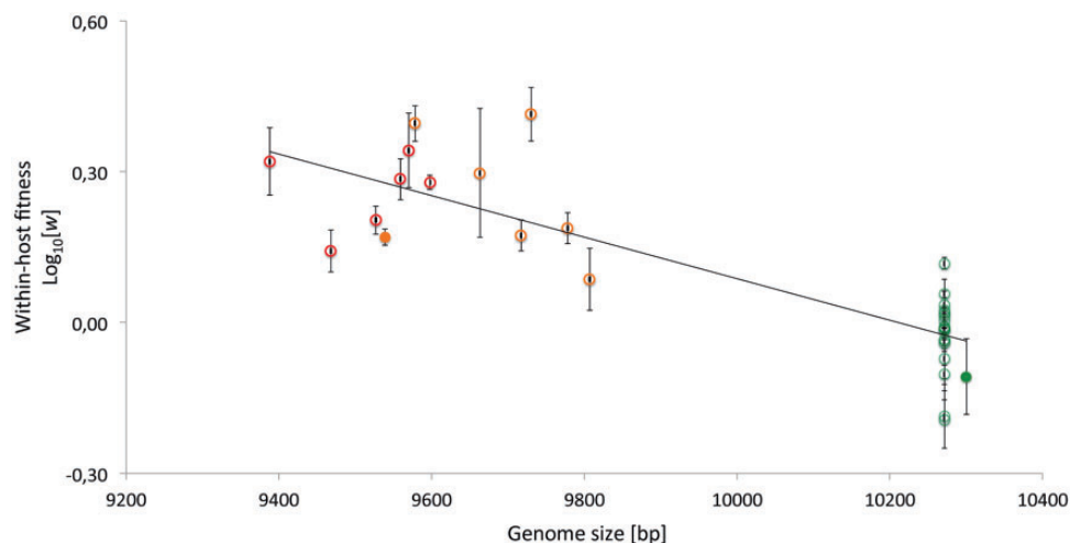
FIG. 7. The relationship between genome size (abscissa) and within-host competitive fitness (ordinate) is given. Green data points indicate no deletions in the heterologous gene (eGFP) were detected, orange indicates part or all of the eGFP was not present, and red indicates part of eGFP and of the viral HC-Pro cistron are not present. The data points for the ancestral TEV-eGFP and TEV have been filled, and TEV-eGFP has been shifted to the right so that it can be easily identified, even though its genome size is the same as other lineages without deletions. A linear regression line has been added only to emphasize the trend in the data. Note that most of the evolved viruses with deletions have a higher fitness than TEV, implicating the observed substitutions with increased fitness.
