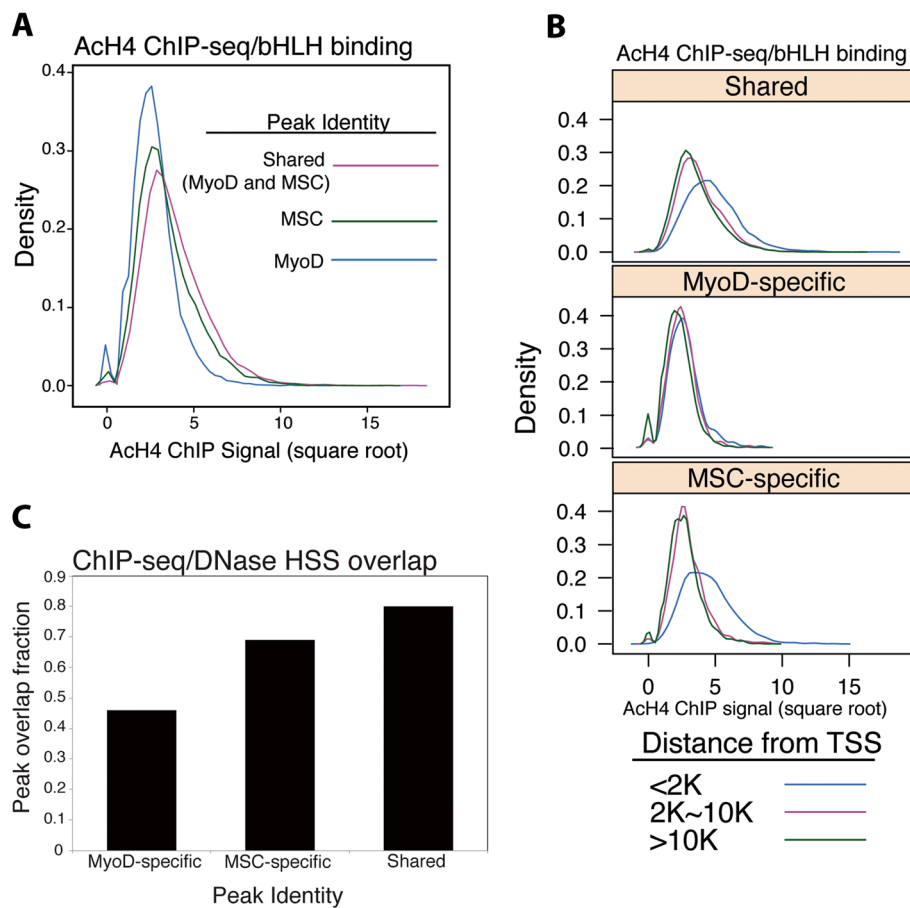
Figure 3 MSC binding is associated with open chromatin. (A) Sites bound by MyoD and MSC are associated with acetylated histones. ChIP-seq for acetylated histone H4 (AcH4) was performed in RD cells and density plots constructed to compare the square root of the AcH4 value at all sites bound by MSC, MyoD or both factors. (B) MSC-specific and MyoD/MS shared peaks are associated with higher levels of AcH4 near the transcription start site (TSS) of genes compared to MyoD-specific peaks. Density plots were constructed as in (A) for categories of peaks first split by peak identity (MyoD, MSC, shared), then subcategorized on distance from the nearest TSS. (C) Sites bound by MSC in RD cells overlap with DNase hypersensitive (HSS) sites in normal human myoblasts. Publicly available DNase HSS data from human myotubes were compared to the sites bound by MyoD and MSC in RD cells. Data for each factor category (for example, MSC-specific) are plotted as the fraction of peaks that overlap with locations that have a signal in the HSS data (that is, the graphed fraction = 1 – fraction of peaks at HSS score of '0'). AcH4, acetylated histone H4; bHLH, basic helix-loop-helix; ChIP, chromatin immunoprecipitation; ChIP-seq, chromatin immunoprecipitation coupled to high-throughput sequencing; HSS, hypersensitive; K, thousands of bp; MSC, myosin; TSS, transcription start site.
