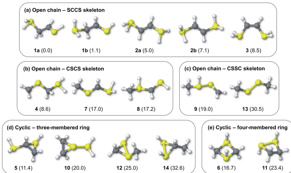
Fig. 2 Optimized C_2H_6S_2^{2+} structures bearing open chain (a) SCCS, (b) CSCS, and (c) CSSC skeleton bonding motifs, and cyclic (d) three- and (e) four-membered rings. The H^{298} values ( \text{kcal mol}^{-1} ) relative to 1a at the CCSD(T)/aug-cc-pVTZ//M06-2X/cc-pVTZ level of theory are shown in parenthesis.
