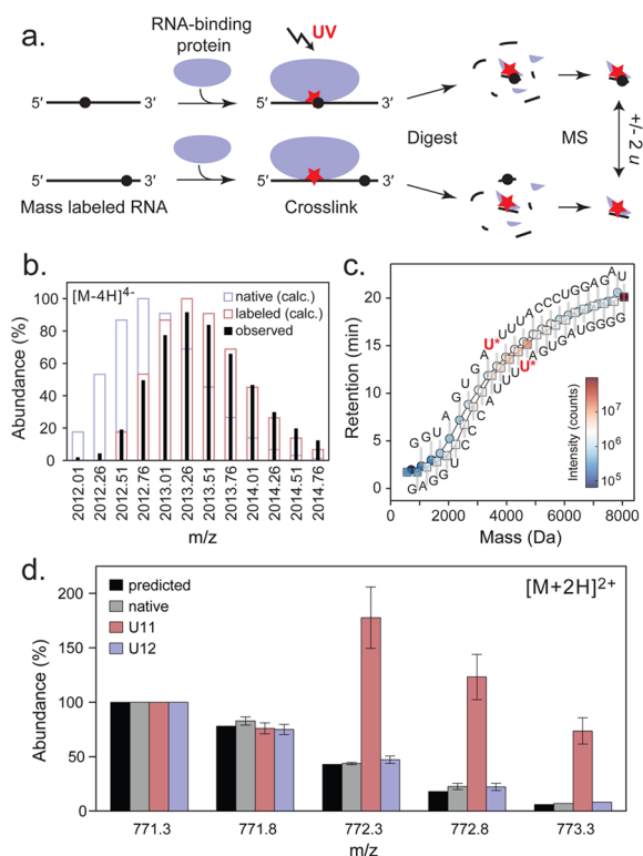
Figure 1. Identifying RNA-protein contacts with site-specific RNA mass labeling. (a) Sample preparation workflow. Oligonucleotides are prepared with selectively enriched ^{18}\text{O} phosphates at distinct positions (black circle), separately incubated with protein, UV cross-linked, hydrolyzed to peptide-nucleotide fragments, and analyzed by MS. (b) Calculated and observed isotopic distributions for [M - 4H]^{4+} ion of 25-nt preE M -let-7f RNA (GGGGUAGUGAU 11 UUUACCCUGGAGAU) labeled with ^{18}\text{O} at the phosphodiester following U11. (c) Direct LC-MS sequencing of U11-labeled RNA, with the mass labeled position indicated as U* (red). (d) Isotope distribution of [MGFGFLSMTAR + UMP + 2H]^{2+} , a tryptic peptide ion derived from cross-linking Lin28A in the presence of preE M -let-7f with natural abundance (native) or ^{18}\text{O} mass labeled at the 3' phosphodiester following U11 or U12. All spectra are normalized to the abundance of the monoisotopic ion 771.3 m/z .
