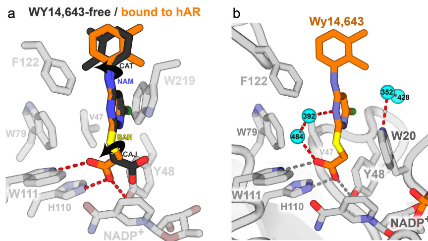
Figure 5. (a) Superposition of free and hAR-bound conformations of the WY 14,643 molecule. The two conformations are superimposed using only the atoms in their the pyrimidine rings. Arrows show the two torsion angles that rotate ~180° upon binding hAR in the ternary complex. (b) Waters (cyan spheres) stabilized by the presence of the WY 14,643 ligand in molA of hAR•NADP + •WY 14,643. The waters shown here are particular to the ternary complex and not observed in the hAR•NADP + binary complex (PDB ID 3Q65). The corresponding water molecules in molB are W390, W386, W396, and W553, respectively.
