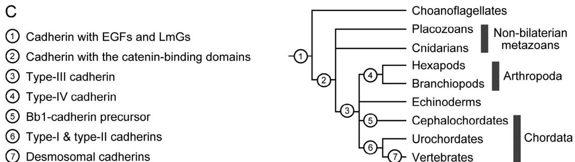
Figure 3. Diversity and evolution of the extracellular domain structures of classical cadherins in the Metazoa. (A) Comparison of the domain structures of selected classical cadherins and a desmosomal cadherin in bilaterian and nonbilaterian metazoan phyla. Gaps (dotted lines) are introduced to highlight homologous extracellular regions between distinct cadherins. (B) Comparison of the domain compositions among the classical cadherin types. (C) A possible phylogenetic diagram showing key genomic changes that contributed to the structural diversification of cadherins at the AJ and the desmosome.
