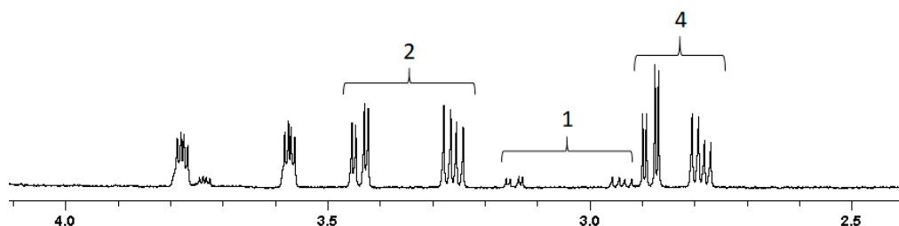
Figure 2. ^1\text{H-NMR} spectra extract (4.2–2.2 ppm) for cystine:sulfite (1:10) with a [\text{SO}_3^{2-}] = 0.1 \text{ M} , after 20 min at pH 8–9 in the region.
