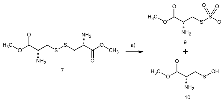
Scheme 3. Reaction performed to obtain desired product 9 , where (a) Na 2 SO 3 (2 eq), H 2 O at r.t.
