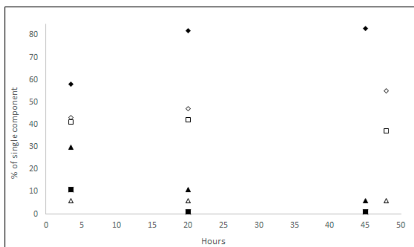
Figure 16. Comparison of temperature effect at pH 4 (▲ cystine 1, □ sulfenic acid 4 and ◇ SSC 2), and at pH 9 (▲ cystine 1, ■ sulfenic acid 4 and ◆ SSC 2).
