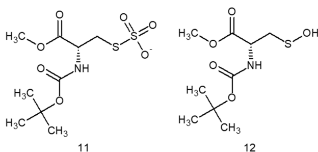
Figure 7. Desired SSC derivatives from compound 8 .
