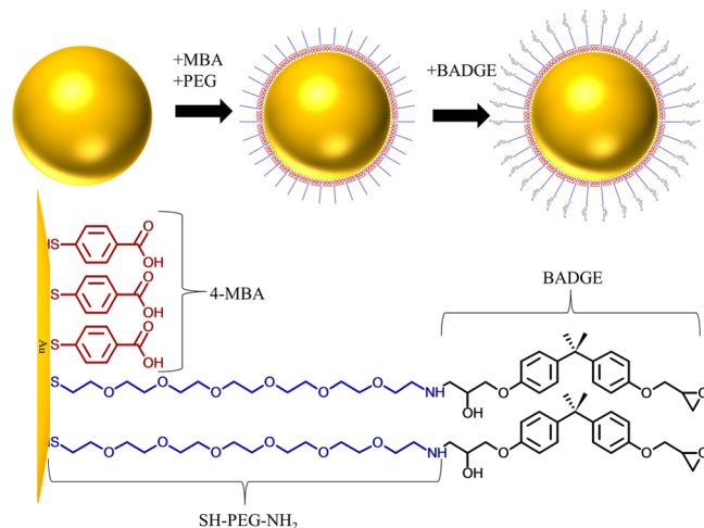
Figure 1. Scheme for the synthesis of BADGE-functionalized SERS nanoprobes. Below: chemical structures of mixed SAM components.
