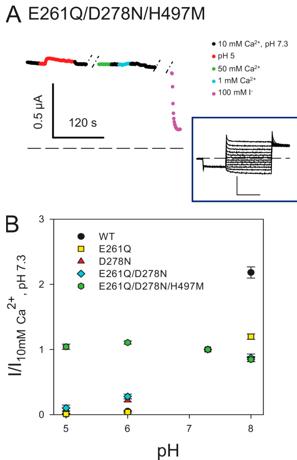
Figure 7. Effect of [H^+]_{ext} on ClC-Ka WT and its mutants E261Q, D278N, E261Q/D278N, and E261Q/D278N/H497M. (A) The current at 60 mV, shown in color, of the triple mutant E261Q/D278N/H497M as a function of time (color code as in Fig. 6). Inset in A shows representative current traces of the mutant in standard solution. Horizontal bars, 100 ms; vertical bars, 1 \mu A. Capacitive transients have been blanked for clarity. (B) Dose-response relationship of the modulation by protons of ClC-Ka WT (black circles; n = 14 ) and the mutants E261Q (yellow squares; n = 4 ), D278N (red triangles; n = 5 ), E261Q/D278N (light blue rhombi; n = 5 ), and E261Q/D278N/E261Q (green hexagons; n = 5 ). Currents at 60 mV were normalized to values measured in standard solution and plotted versus pH. Data for WT are different compared with Fig. 2 because they were obtained from different oocytes as control measurements in the mutagenic screen.
