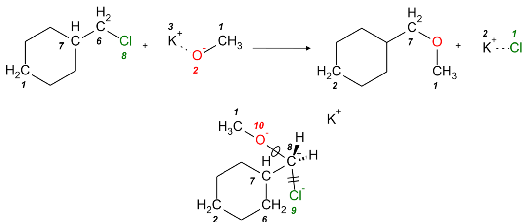
Fig. 4: A substitution reaction with an imaginary transition structure.
