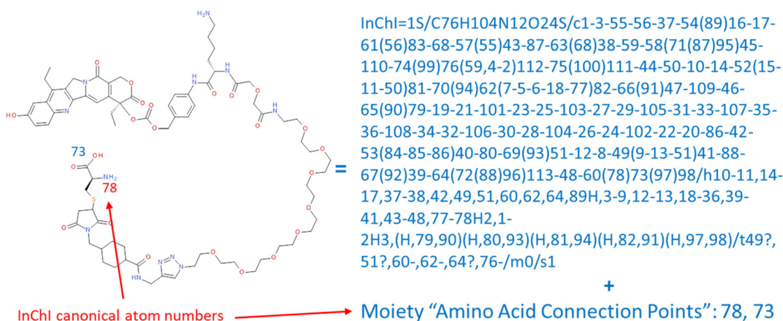
Fig. 1: Definition of substituents via InChI canonical atom numbers.
