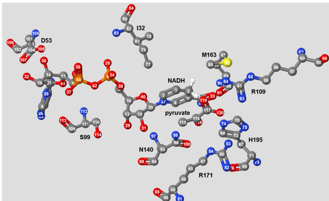
Fig. 2: Intermediate complex of LDH, NADH and pyruvate.
