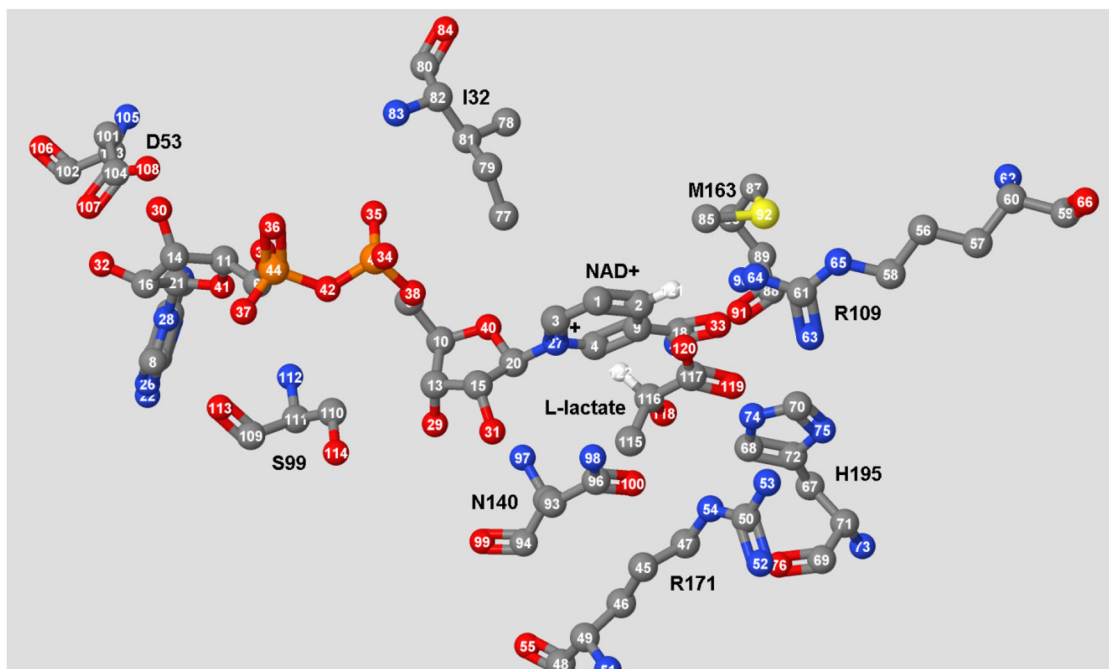
Fig. 3: Intermediate complex of LDH, \text{NAD}^+ and L-lactate.
