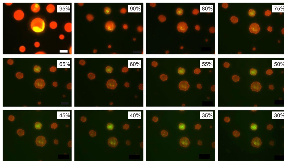
Figure 6. Fluorescence images of model droplets exposed to decreasing relative humidity. A droplet contains water, NaCl, mucin (red), and DDPC (green). DDPC: 1,2-dihexadecanoyl- sn -glycero-3-phosphocholine. Reprinted with permission from Vejerano and Marr. 50 Copyright (2018) The Royal Society.
