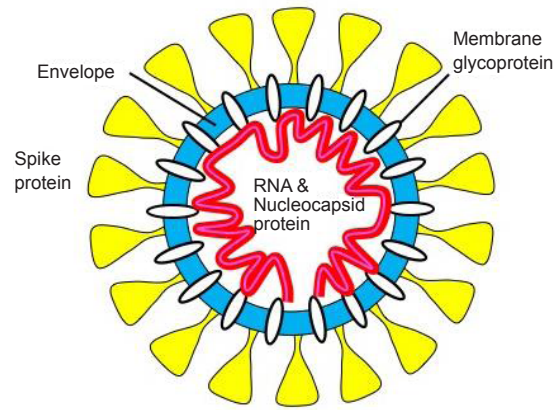
Figure 2. Structure of a coronavirus particle.
