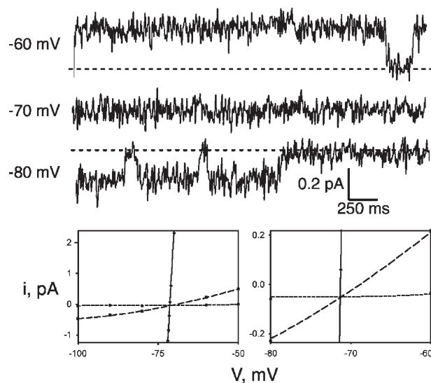
Figure B1. Single KcsA-E71A channels were recorded as in the main text, with 200 mM K^+ in/10 mM K^+ and 190 mM Na^+ out. 10 \mu M Ba^{2+} was also included in the internal solution to produce block events. Immediately after recording a single-channel I-V curve, 25 \mu M valinomycin was added to the bilayer to raise the conductance \sim 100 -fold, and the macroscopic I-V curve was measured within a minute. (Top) Illustrative records (filtered at 50 Hz) at voltages on either side of the reversal potential before the addition of valinomycin. Dashed line marks zero-current level. (Bottom) I-V curves for open channel (squares), blocked channel (circles), and valinomycin (diamonds). Curves (dashed for channel, solid for valinomycin) are third-order polynomial fits to the data points. Reversal potential is the voltage at which the open-channel or valinomycin curve crosses the blocked-channel curve. Right panel is a blown-up view of left panel.
