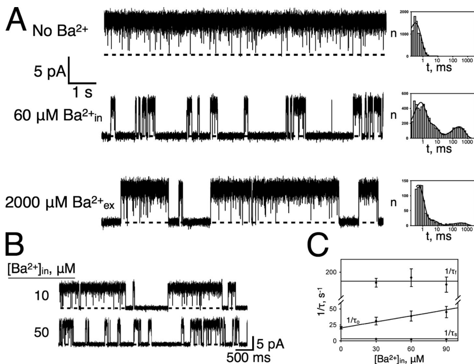
Figure 3. \text{Ba}^{2+} block of KcsA-E71. Single-channel recordings were collected at 50 mV with 200 mM of internal \text{K}^+ /20 mM of internal \text{K}^+ , with or without \text{Ba}^{2+} as indicated. (A) \text{Ba}^{2+} blocks from either side of the membrane. Nonconducting dwell-time histograms (log-binned) are shown in each condition, along with exponential fits. Time constant for zero \text{Ba}^{2+} is 0.4 ms; time constants of triple-exponential fits for internal \text{Ba}^{2+} are 0.9, 6, and 370 ms, and for external \text{Ba}^{2+} are 0.3, 5, and 350 ms, respectively. (B and C) Bimolecular behavior of \text{Ba}^{2+} block. Representative recordings at two concentrations of internal \text{Ba}^{2+} are shown along with plots of inverse time constants for unblocked times ( 1/\tau_0 ) and fast and slow block times. Second-order rate constant for \text{Ba}^{2+} association derived from slope of unblocked-time data is 2.9 \times 10^5 \text{ M}^{-1}\text{s}^{-1} .
