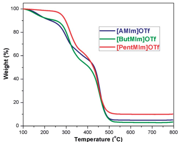
Fig. 1 TGA curves of [AMIm]OTf, [ButMIm]OTf, and [PentMIm]OTf.
