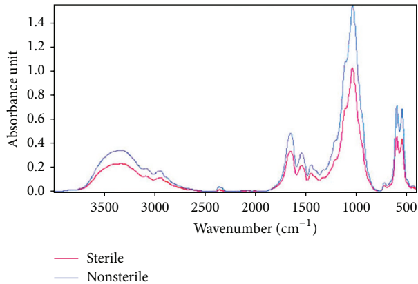
FIGURE 2: FTIR spectra of the sterile and nonsterile collagen/ \beta -TCP scaffolds.
