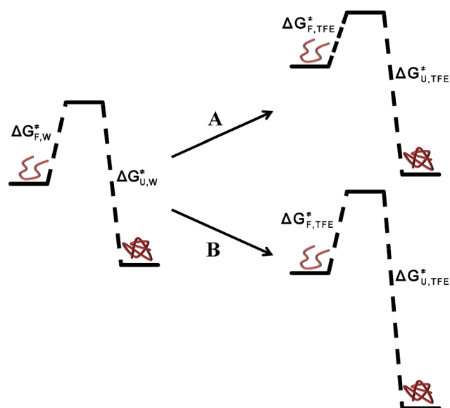
Figure 4. Cartoon illustration of the effect of TFE on the folding and unfolding free energy barriers of pKID. In scenario A, \Delta G_{U,W}^{\ddagger} > \Delta G_{U,TFE}^{\ddagger} and \Delta G_{F,W}^{\ddagger} = \Delta G_{F,TFE}^{\ddagger} , whereas in scenario B \Delta G_{U,W}^{\ddagger} = \Delta G_{U,TFE}^{\ddagger} and \Delta G_{F,W}^{\ddagger} < \Delta G_{F,TFE}^{\ddagger} .
