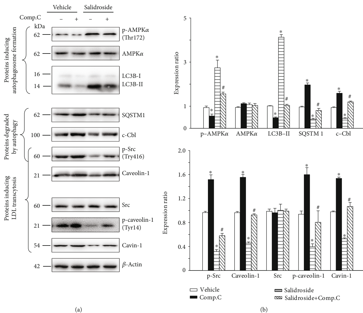
FIGURE 6: Compound c prevents salidroside-induced autophagic degradation of p-Src and caveolin-1. HUVECs were treated with indicated concentration of salidroside ( 1 \mu\text{M} ) for 3 h in the presence or absence of compound c ( 10 \mu\text{M} , 3 h). Whole-cell lysates from HUVECs were subjected to western blot analyses for indicated proteins, with \beta -actin as a loading control. Representative western blotting analyses of the indicated proteins (a) and summary bar graph showing the expression of the indicated proteins (b). n = 3 , *p < 0.05 versus vehicle. \#p < 0.05 versus salidroside ( n = 3 ).
