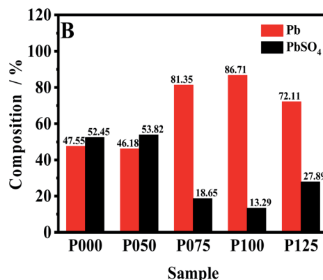
Fig. 7 XRD patterns (A) and compositions (B) of the NAMs collected from the interior of negative plates after the HRPSoC cycle-set.
