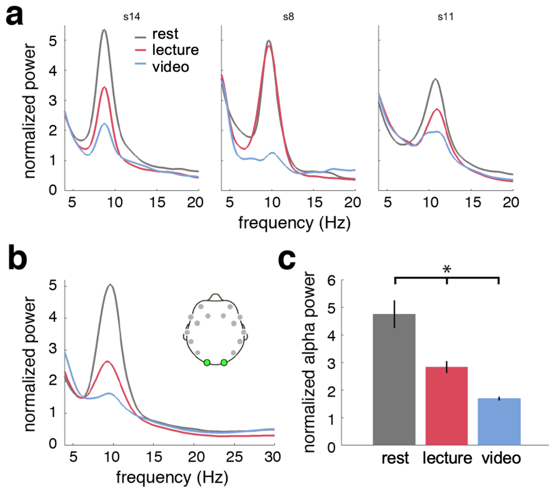
Fig. 2. Alpha power per condition. (A) Power spectra (averaged over occipital sensors, see inset in panel B) of three representative example subjects for each of the conditions of interest (resting state in gray, lecture in pink and video in blue), showing clear peaks in the alpha band. (B) Similar as in A, averaged over all subjects ( N = 22 ), including all available recording sessions per subject. (C) A significant ( P < 0.001 ) decrease of posterior alpha power over conditions (computed in 1 Hz band centered at individual alpha peak frequency for each subject, normalized with average power in the spectrum per channel). Error bars indicate standard error of the mean (SEM; N = 22 ).
