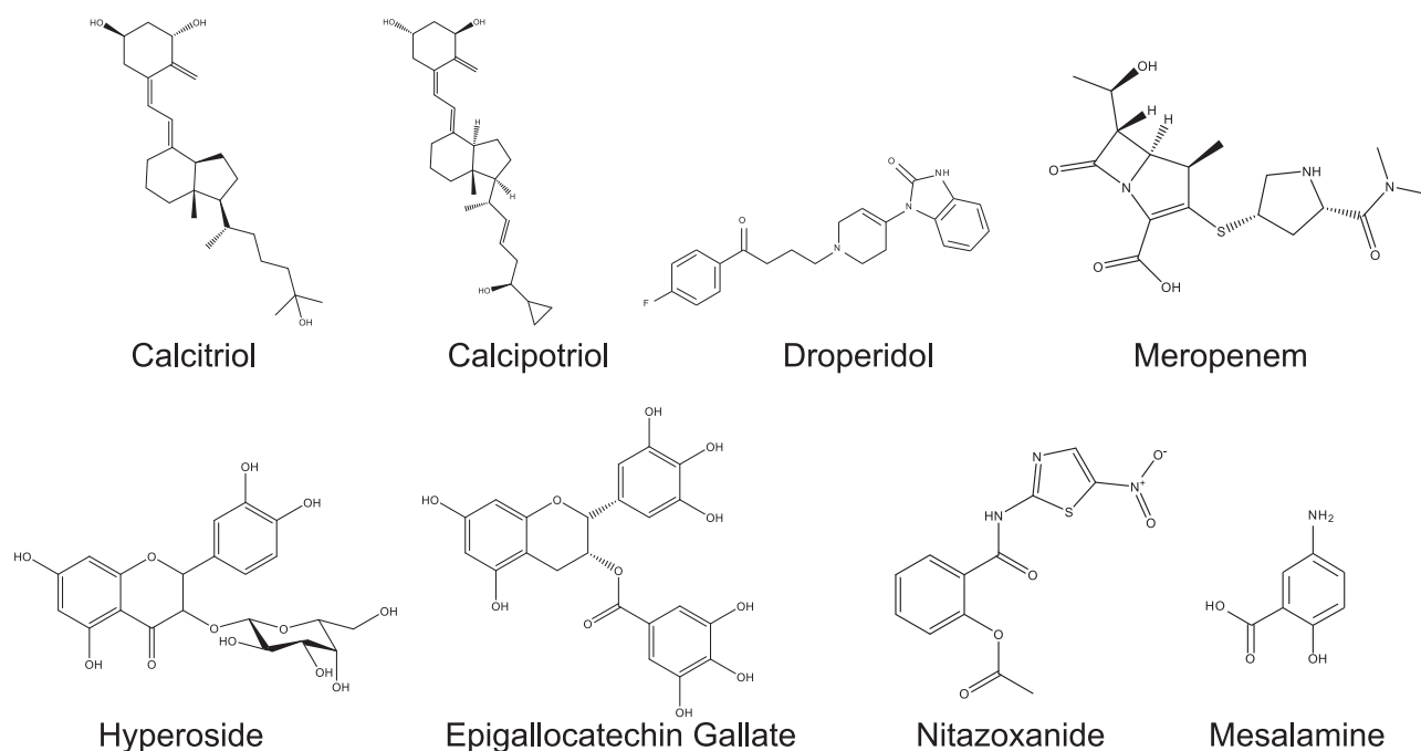
Fig. 1. Chemical structures of the test compounds.
