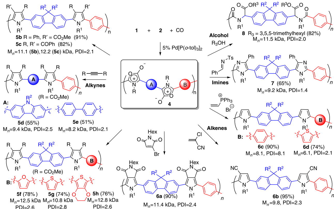
Figure 5 | Transformation of poly-Münchnones into families of conjugated polymers. Derivatization performed on poly-Münchnone samples of 8–12 kDa to ensure full solubility of 4a–e , and allow the quantification of the cycloaddition.
