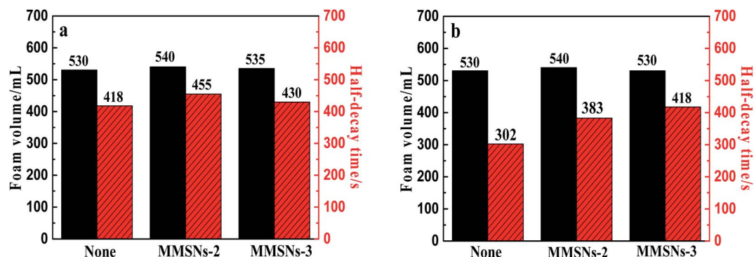
Fig. 10 Foam performance of (a) pure SDS solutions (b) oil/SDS solution with MMSNs.
