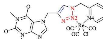
C22H22ClN8O6Re
