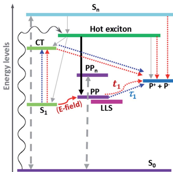
Fig. 6 Schematic energy diagram (not to scale) depicting physical processes contributing to the dynamics of photoinduced absorption measured at 638 nm in 1 : 1 and 2 : 1 P3HT:PCBM solar cell devices under the influence of applied electric fields for 12 and 24 \mu\text{J cm}^{-2} initial pump pulse (520 nm) excitation fluence. S_0 : electronic ground state; S_1 : (thermalized) singlet exciton; S_n : high-energy exciton; CT: charge transfer exciton; PP: polaron-pair; LLS: long lived states; PP_n : high-energy PP state; P^+ + P^- : polaron states. Black line: ultrafast formation of nascent PPs; dotted blue lines: pump-initiated processes without electric field; dashed grey lines: bimolecular annihilation processes; red lines: electric-field-influenced processes; t_1 : PP decay in the absence of any electric field; \tau_1 : PP decay occurring with the influence of an electric field. The energy levels given are only schematic and the energy scale is therefore not reflecting quantitative values. See text for more details.
