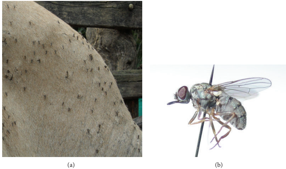
FIGURE 2: Potential role of Haematobia sp. (a) Common level of infestation by Haematobia sp. on the back of a cattle, Thailand (one Stomoxys sp. also visible); (b) Haematobia species (2.5–4 mm).
