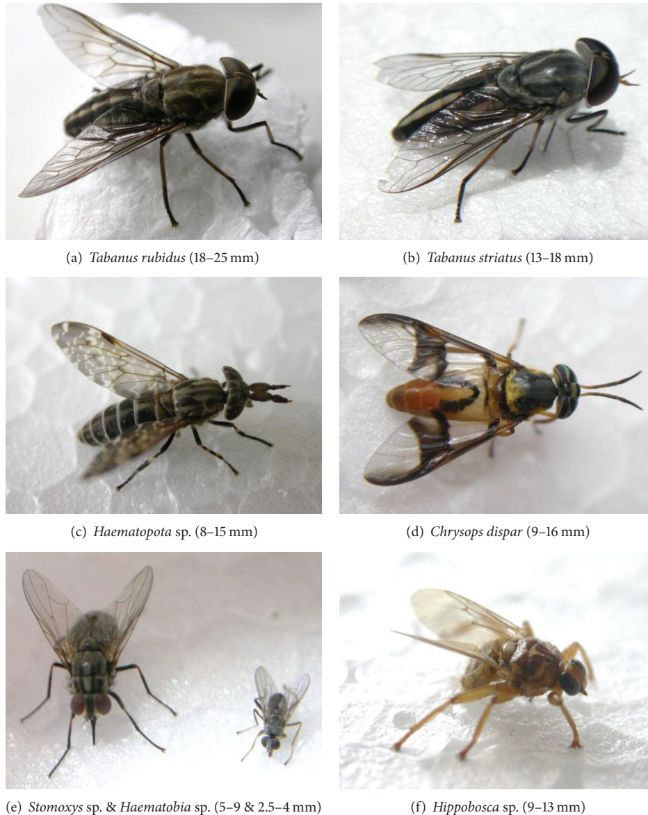
FIGURE 1: Some of the potential vectors of Trypanosoma evansi in Thailand.
