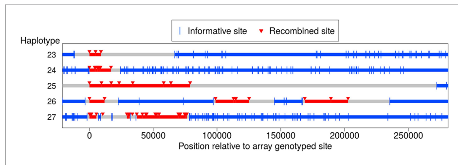
Figure 5. Long-range recombination events observed in sequence data. Shown are three contiguous recombination tracts with length \geq 9 kb, \geq 16.9 kb, and \geq 79 kb as well as two sets of clustered long-range recombination events that span \sim 200 kb and \sim 76 kb.
