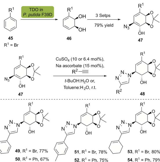
Scheme 5 Chemo-enzymatic synthesis of the bromoazidocondurititol derivative, and synthesis of triazolyconduritols.
