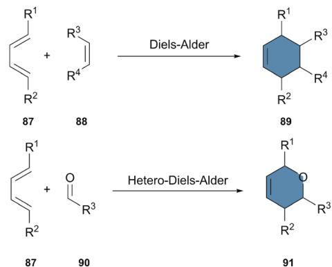
Scheme 11 Diels–Alder reaction and hetero-Diels–Alder reaction.
