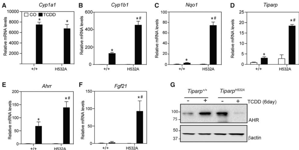
Figure 5. Increased hepatic gene expression of aryl hydrocarbon receptor (AHR)-regulated genes. Mice were treated with a single injection of 10 \mu g/kg 2,3,7,8-tetrachlorodibenzo- p -dioxin (TCDD), or corn oil (CO) (vehicle) alone, and euthanized 6 days later. RNA and real time-quantitative PCR for (A) Cyp1a1 , (B) Cyp1b1 , (C) Nqo1 , (D) Tiparp , (E) Ahrr , and (F) Fgf21 were performed as described in the materials and methods section ( n=5 ). G , Representative western blot ( n=3 ) of hepatic AHR protein levels in Tiparp +/+ and Tiparp H532A mice 6 days after treatment with 10 \mu g/kg TCDD or CO (vehicle). * p < .05 2-way ANOVA followed by Sidak's post hoc test compared with genotyped-matched control-treated mice. # p < .05 2-way ANOVA followed by Sidak's post hoc test compared with time-matched TCDD-treated Tiparp +/+ mice. Figure depicts the mean \pm SEM.
