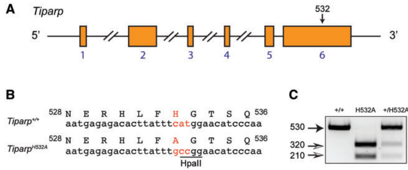
Figure 1. Generation of Tiparp H532A catalytic mutant mice using CRISPR/Cas9-mediated gene editing. A, Schematic diagram of Tiparp wildtype allele with exons, and the approximate location of H532, which was targeted to create a Tiparp H532A mutant mouse. Exons are indicated by the orange boxes and their numbers are indicated in blue font. B, To simplify genotyping, an Hpa II restriction enzyme site was introduced simultaneously with the replacement of histidine 532 with alanine. C, Representative genotyping of wildtype, H532A mutant, and heterozygous mice.
