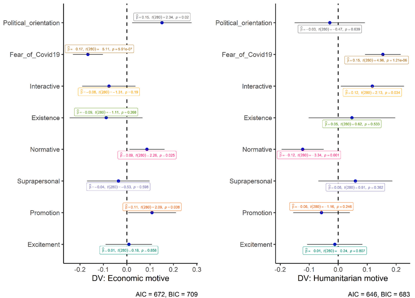
Fig. 2. Unstandardised regression coefficients. Error bars represent 95%-CIs.
