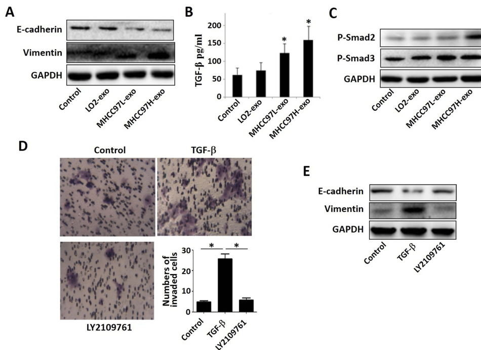
Figure 3 TGF- \beta pathway activated by exosomes derived from HCC cell. Notes: (A) The expression of E-cadherin and Vimentin were detected by Western blot. (B) TGF- \beta concentrations were determined by ELISA kits, treatment with HCC-exosomes for 48 hrs increased TGF- \beta level in cell culture supernatant compared with that in the control group. (C) The expression of p-Smad2 and p-Smad3 were detected by Western blot. (D) Results of transwell invasion assay. The number of positive cells penetrating the pores of the HCC cells treated with the TGF- \beta group was significantly higher than that of the control group and the LY2109761 (TGF- \beta inhibitor) group (* P <0.05). (E) Western blot analysis confirmed the exosomal TGF- \beta efficiency by LY2109761, the expression of E-cadherin decreased and Vimentin expression increased after application. Abbreviation: HCC, hepatocellular carcinoma.
