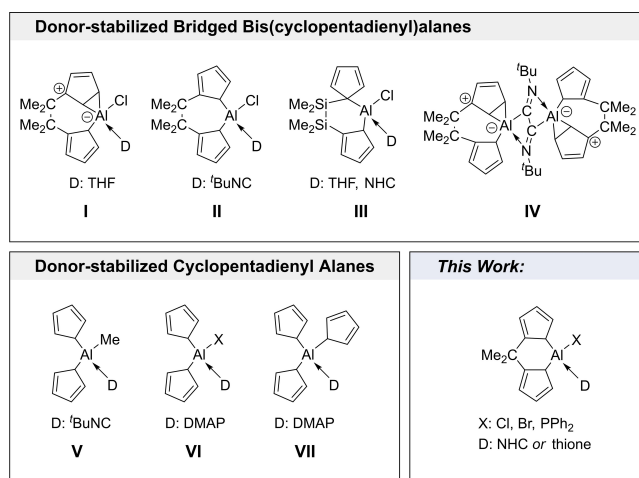
Figure 1. Selected examples of cyclopentadienyl-substituted aluminum donor complexes.
