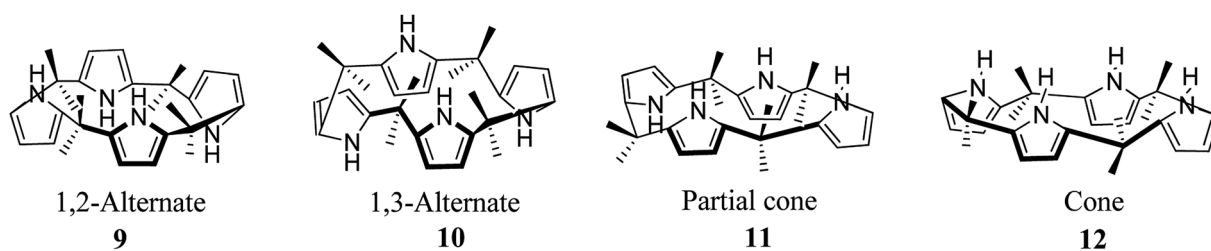
Fig. 2 Different conformations of C4P.
