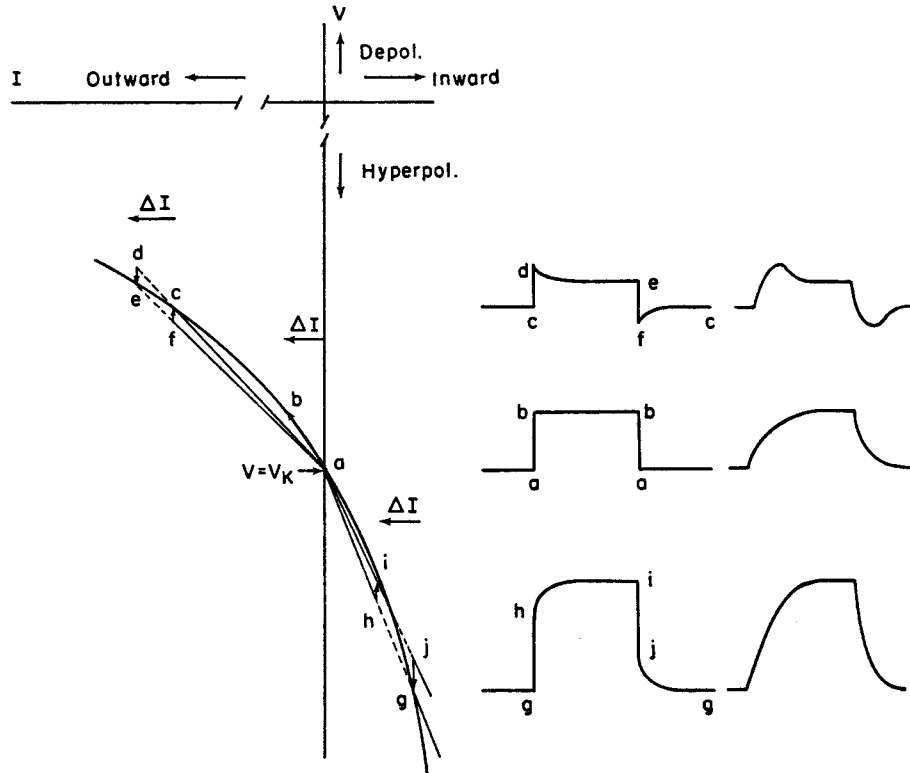
FIGURE 12. I, V steady-state plot showing, qualitatively, the properties of the potassium current system in squid axon is seen on the left. Note, breaks are shown in the I and V axes to remind the reader that we are considering the I, V plot at a highly expanded scale in order to examine the "linear" (small-signal) response of \Delta V with an applied \Delta I . The response in time to a pulse of current \Delta I at the different resting states, depicted by the points c, a, and g , is shown in the middle column. To the extreme right the corresponding response is shown when the membrane capacitance is added in parallel.
