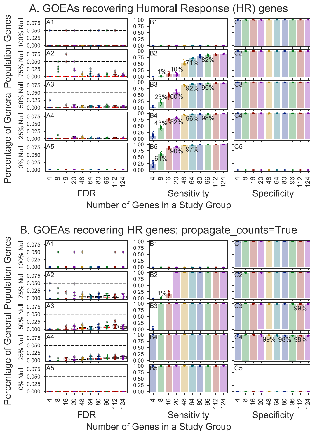
Figure 3. Results for 20,000 GOATOOLS GOEA stochastic simulations with varying sensitivity and consistently high specificity. GOEAs performed well on study groups of 8+ genes if the GOATOOLS GOEA option propagate_counts set to True.
