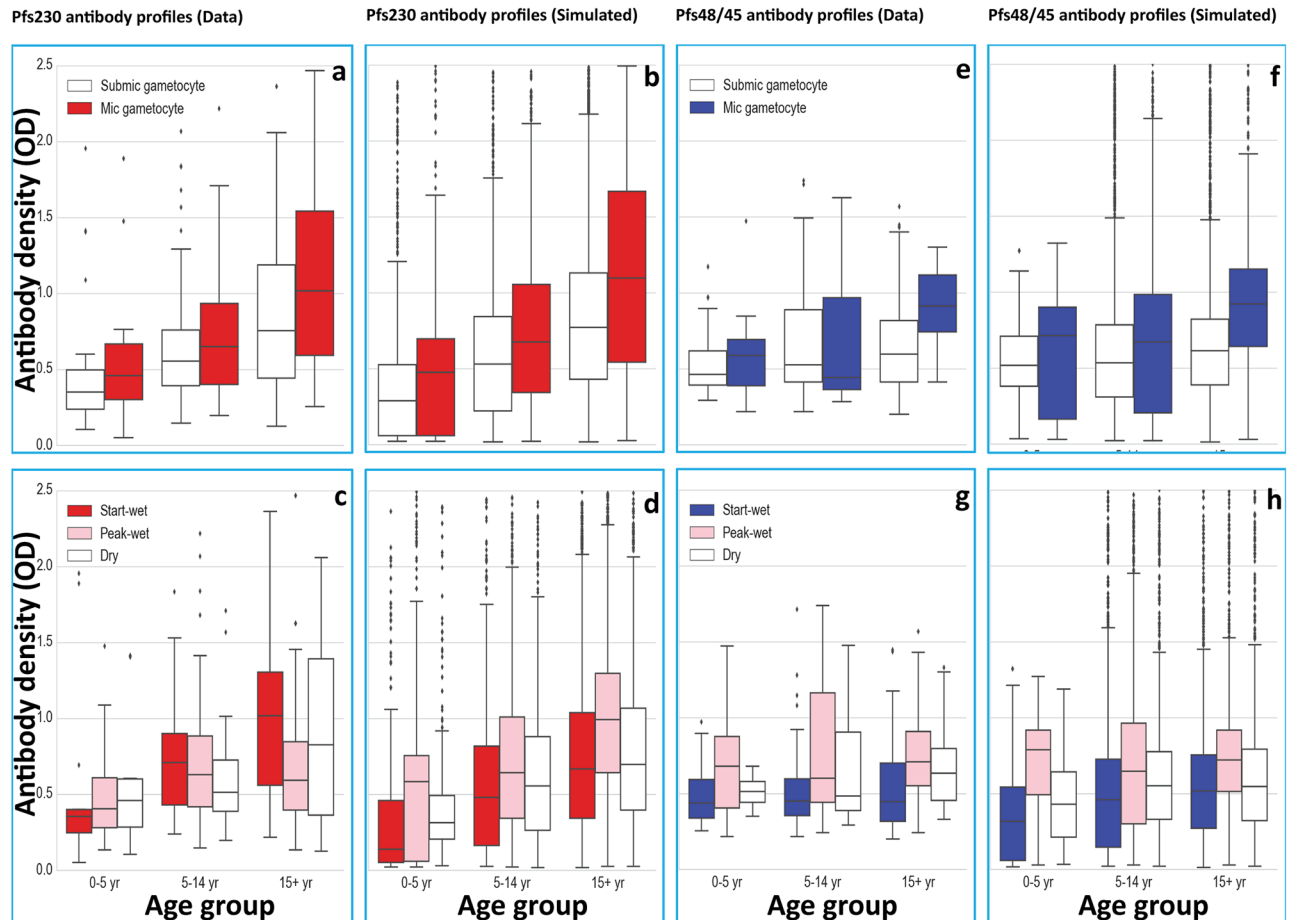
Fig 2. Dynamics of Pfs230 and Pfs48/45 antibody densities by age, season and gametocyte density. Submic gametocyte = Submicroscopic gametocyte densities ranging from 0.01–4 gametocytes/ \mu\text{L} blood thus negative by microscopy and positive by QT-NASBA. Mic gametocyte = gametocyte positive by both microscopy and QT-NASBA. Antibody densities of field study participants were measured in subsamples of n = 37 , n = 97 and n = 157 samples in age groups 1–4, 5–14 and \geq 15 years of age respectively and shown in panel a for Pfs230 and panel e for Pfs45/45. Antibody densities of simulated individuals were measured in subsamples of n = 1500 , n = 3000 and n = 10500 samples in age groups 1–4, 5–14 and \geq 15 years of age respectively and shown in panel b for Pfs230 and panel f for Pfs48/45. Antibody densities of field study participants were measured in subsamples of n = 102 , n = 96 and n = 93 samples during the start, peak and wet seasons respectively and shown in panel c for Pfs230 and panel g for Pfs45/45. Antibody densities of simulated individuals were measured in subsamples of n = 5000 , n = 5000 and n = 5000 samples during the start, peak and wet seasons respectively and shown in panel d for Pfs230 and panel h for Pfs48/45. Error bars show horizontal lines from top indicating maximum antibody density, 75% percentile, median (50% percentile), 25% percentile and minimum antibody density. Dots outside shaded boxes represent outliers in the distribution of antibody densities within the given subsample.
