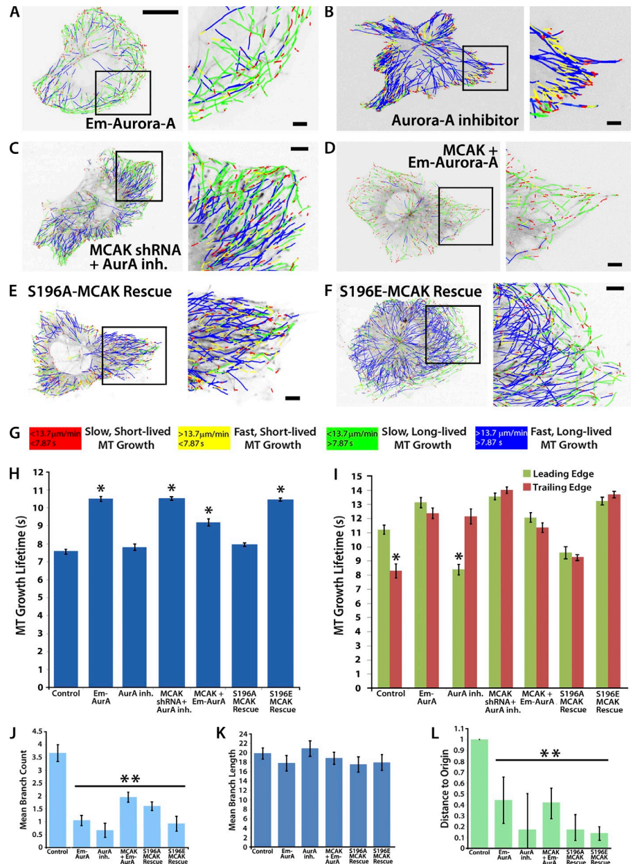
Figure 5. Aurora A rescues MCAK over-expression and promotes long-lived MT growth at the leading edge. (A–F) Overlays of MT growth tracks from 2-min time-lapse videos of mApple-EB3 (2-s intervals) from plusTipTracker software in whole cells (left), and zoom of black-boxed regions (right) of HUVECs over-expressing Em–Aurora A in cells treated with 40 nM Aurora A inhibitor, in MCAK knock-down cells treated with Aurora A inhibitor, in cells coexpressing mCherry-MCAK and Em–Aurora A, or in shRNA-treated HUVECs rescued with MCAK S196A or S196E mutant constructs. MT tracks are color coded according to their growth speed and lifetime (color scheme in G). (H–L) Comparison of parameters for MT and cell behavior for the treatments of HUVECs described in A–F. Comparison of mean MT growth excursion lifetimes in whole cells (H) and within the leading and trailing edges of wound-edge HUVECs (I). Quantification of branch number (J) and length (K) in HUVECs cultured on fibronectin-coupled 0.7-kPa polyacrylamide substrates to promote branching morphologies. (L) Quantification of directional HUVEC migration in wound-edge migration assay. Bars: (main) 10 \mu\text{m} ; (zoomed) 2 \mu\text{m} . *, P < 0.001 ; **, P < 0.05 . Error bars show \pm standard error in H and I and \pm standard deviation in J–L.
