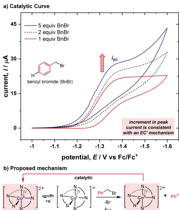
Fig. 2 (a) Increment of forward current for the \text{Co(II)/Co(I)} couple ligated by BPP 3 with successive increases in benzyl bromide concentration, consistent with an \text{EC}' mechanism. CVs run with 1.0 mM \text{CoBr}_2 with 2.0 mM 3 at varying equivalents of benzyl bromide in a 100 mM solution of \text{Bu}_4\text{NPF}_6 in acetonitrile, using a 0.071 \text{ cm}^2 boron-doped diamond working electrode at a scan rate of 0.10 \text{ V s}^{-1} . CVs are plotted in polarographic notation with positive currents corresponding to reduction. (b) Proposed \text{EC}' mechanism.
