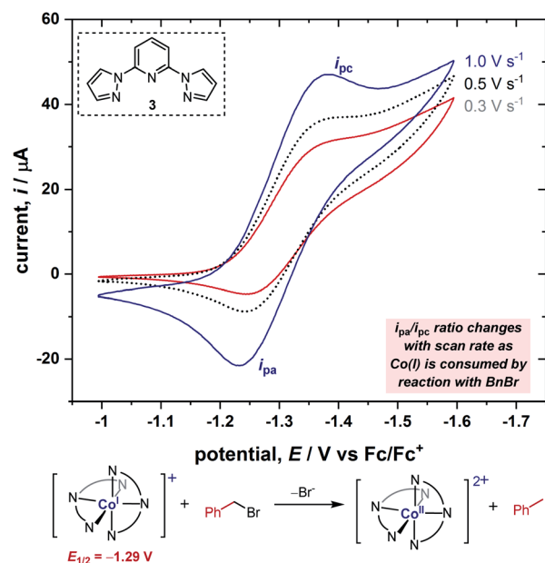
Fig. 3 The variation in peak-current ratio ( i_{pa}/i_{pc} ) as a function of scan rate enables measurement of the rate constant of oxidative addition occurring during the CV scan. CVs of 1.0 mM \text{Co(II)} complex with 2.0 mM BPP ligand 3 in the presence of 1.0 mM benzyl bromide at varying scan rates in a 100 mM solution of \text{Bu}_4\text{NPF}_6 in acetonitrile, using a 0.071 \text{ cm}^2 boron-doped diamond working electrode. CVs are plotted in polarographic notation with positive currents corresponding to reduction.
