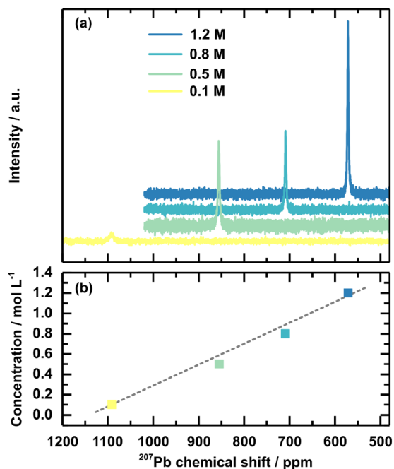
Fig. 5 207 Pb NMR spectra (a) of the 3CatPbBr 3 solution concentration series and an additional diluted 0.1 M solution. (b) Visualises the dependency of the 207 Pb chemical shift on the concentration. The grey dashed line gives a guide for the eye of the linear dependency.
