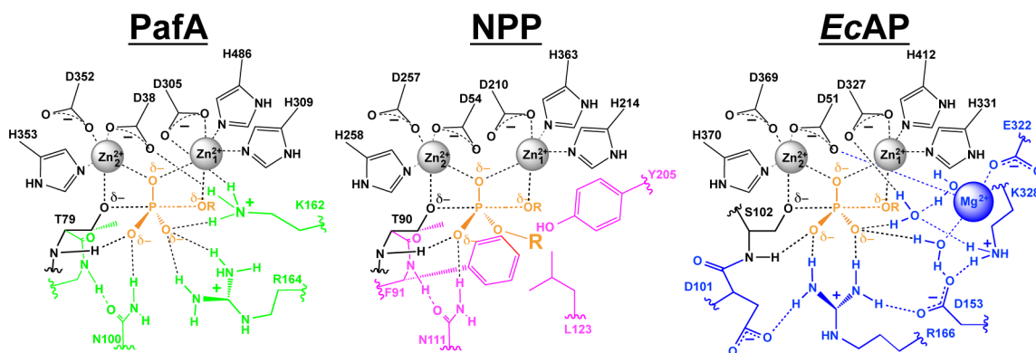
Figure 2. Active-site schematics for PafA, NPP, and EcAP. The enzymes have a conserved bimetallo core (black, including the threonine or serine nucleophile), conserved zinc ligands (gray), and additional non-universally conserved active-site residues, which are colored for each enzyme. The phosphoryl group, in orange, is shown with partial bonding to the nucleophile and its leaving group (OR), corresponding to the reaction's presumed transition state.
