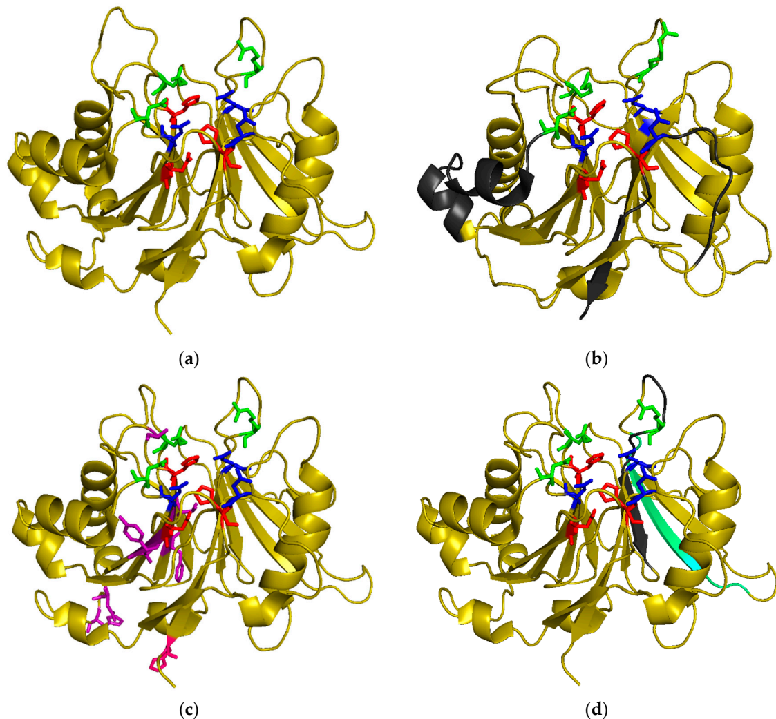
Figure 2. 3D structure of CdtBs: catalytic residues are represented in red, metal binding residues in blue and substrate binding residues in green. (a) HducCdtB (PDB accession number: 1sr4); (b) EcolCdtB-II (PDB accession number: 2f1n) with putative NLS regions in grey; (c) AactCdtB (PDB accession number: 2f2f) with residues potentially involved in phosphatase activity in purple and the H281 activating residue in pink; (d) AactCdtB (PDB accession number: 2f2f) with putative nuclear localization signal region in grey and cholesterol recognition sequence in cyan.
