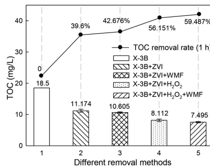
Fig. 10 TOC removal rate of X-3B under different removal methods (pH 4.0, 8 mM H 2 O 2 , 50 mg L -1 X-3B, 0.5 g L -1 Fe 0 , and T = 25 °C).
