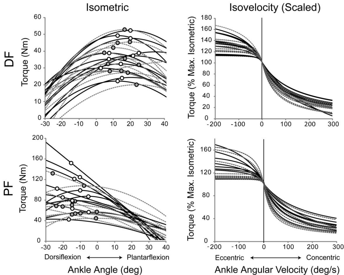
Figure 3. Equations representing the best fit between the experimental data and second order polynomials (torque-angle relation; isometric) and rectangular hyperbolas (torque-angular velocity relation; isovelocities) for young (solid black lines) and older (dashed gray lines). The solid circles positioned on the isometric curves represent the peak isometric torque. For some subjects, the peak did not occur within the subject's range of motion, in these cases the solid circle is positioned at the end of the range of motion. The isovelocities fits are scaled to the peak isometric torques. doi:10.1371/journal.pone.0015953.g003
