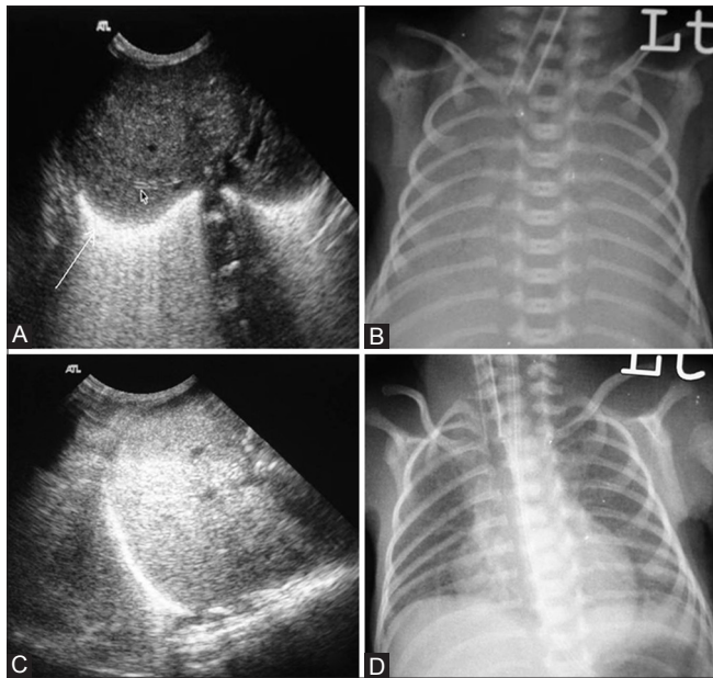
Figure 3 (A-D): A 6-hour-old girl born at 28+6 weeks of gestation having respiratory distress soon after birth. Axial TASL (A) shows an HMD pattern. Corresponding chest radiograph (B) taken on day 1 showed bilateral whiteout lungs consistent with hyaline membrane disease. Coronal TASL (C) at day 14 showed resolution of HMD pattern with corresponding chest radiograph (D) showing normalization (Group 2)
