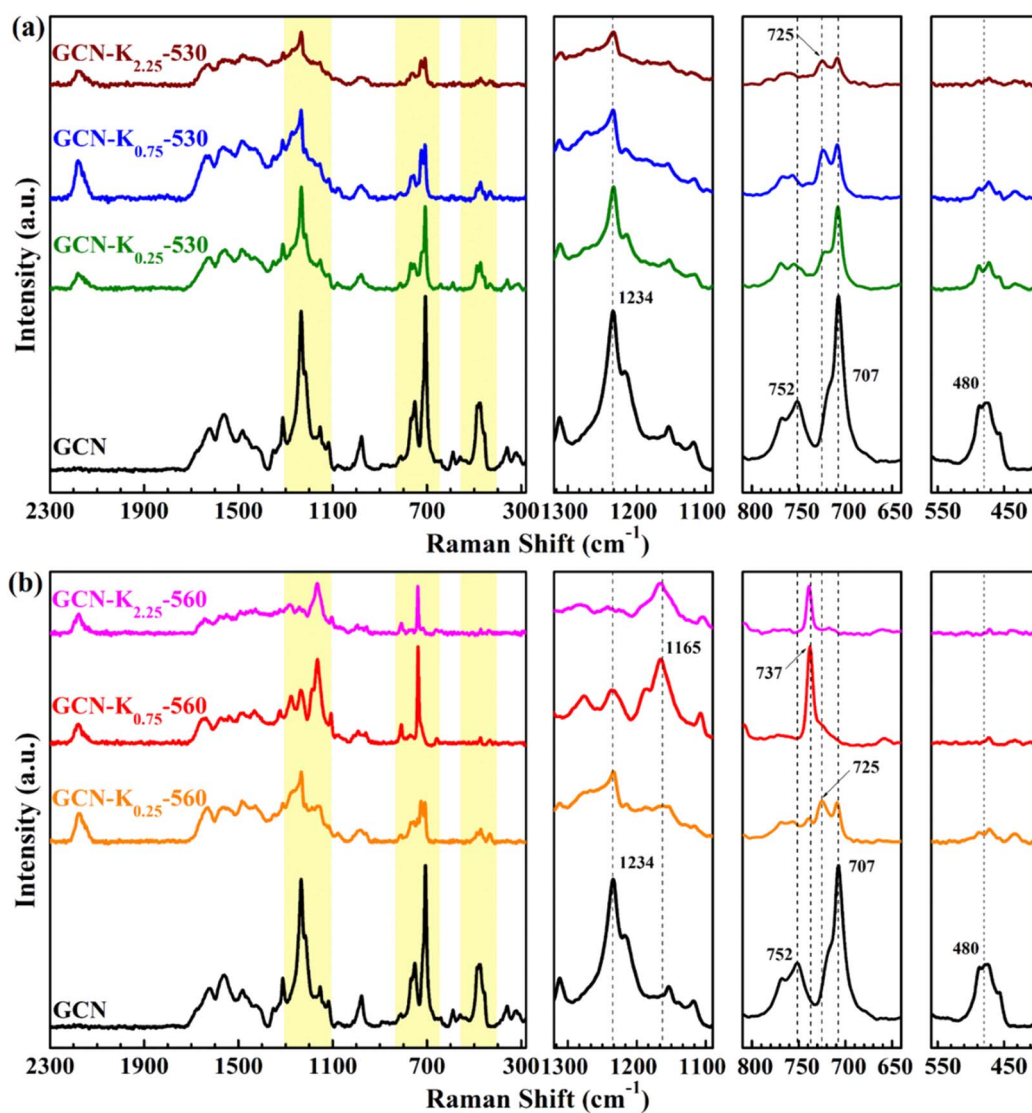
Fig. 4 Raman spectra (1064 nm excitation) of GCN and K + -doped GCNs at 530 °C (a) and 560 °C (b).
