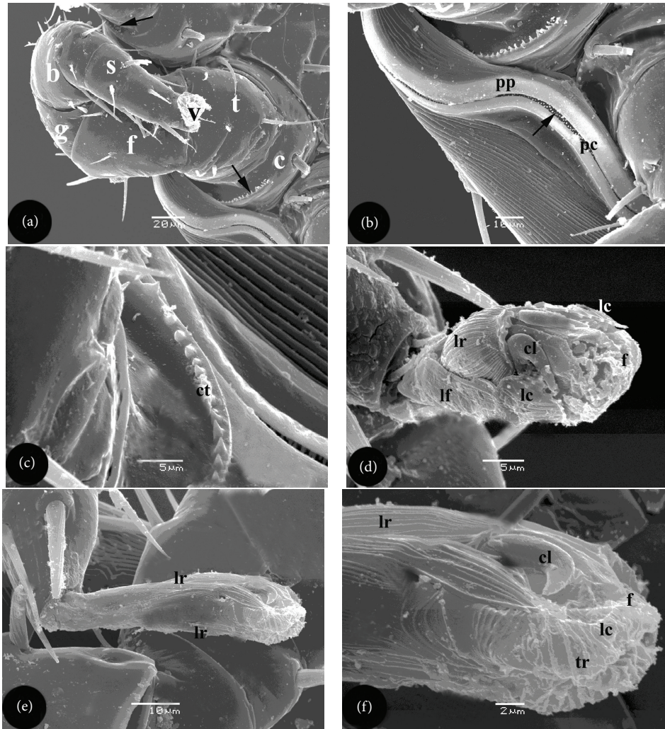
FIGURE 3: Scanning electron micrographs of peritreme and pulvilli of female L. nuttalli . (a) The second leg, consisting of 6 segments, namely, coxa (c), trochanter (t), femur (f), genu (g), tibia (b), and tarsus (s) terminating with pulvillus (v), beside the peritreme. The coxa carries a row of minute conical tubercles (arrow) near the peritremal plate (pp). (b) Peritremal plate (pp) surrounding peritremal canal (pc) which contains minute papillae. (c) Higher magnification of the row of minute conical tubercles (ct) on the coxa. (d) Pulvillus of the first leg carrying 2 curved claws (cl), ventral longitudinal ribs (lr), two lateral laciniae (lc), and overlapping terminal integumental folds (f). (e) Pulvilli of 2nd–4th legs showing longitudinal integumental ridges (lr) on dorsal and ventral sides. (f) As in (e) showing terminal medioventral claws (cl), lateral laciniae (lc), and transverse ridges (tr).
