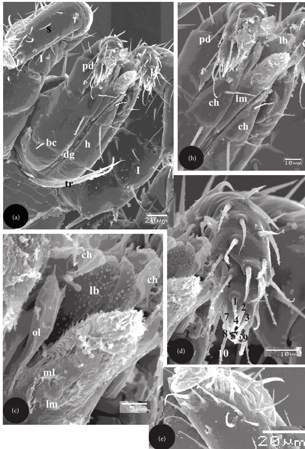
FIGURE 2: Scanning electron micrographs of gnathosoma and sense organs of female L. nuttalli . (a) Whole gnathosoma consisting of long basis capituli (bc) carrying median hypostome (h) and 2 lateral pedipalps (pd). Tritosternum (tr) with 2 laciniae located below the deutosternal groove (dg) on the ventral side of the basis capituli. I = first leg, s = tarsus. Arrows showing spines in the deutosternal groove. (b) Hypostome carrying dorsal labrum (lb), ventral labium (lm), and 2 lateral chelicerae (ch). Pd = pedipalp. (c) As in (b) showing labrum (lb) consisting of 2 lobes, each carrying minute papillae, terminal segments of chelicerae (ch), and labium consisting of club-shaped outer lobes (ol) and 2 median lobes (ml) carrying laciniae (arrows). (d) Palpal organ (po) consisting of 10 terminal setae (1–10). (e) Foreleg tarsal organ (to) consisting of 15 terminal setae.
