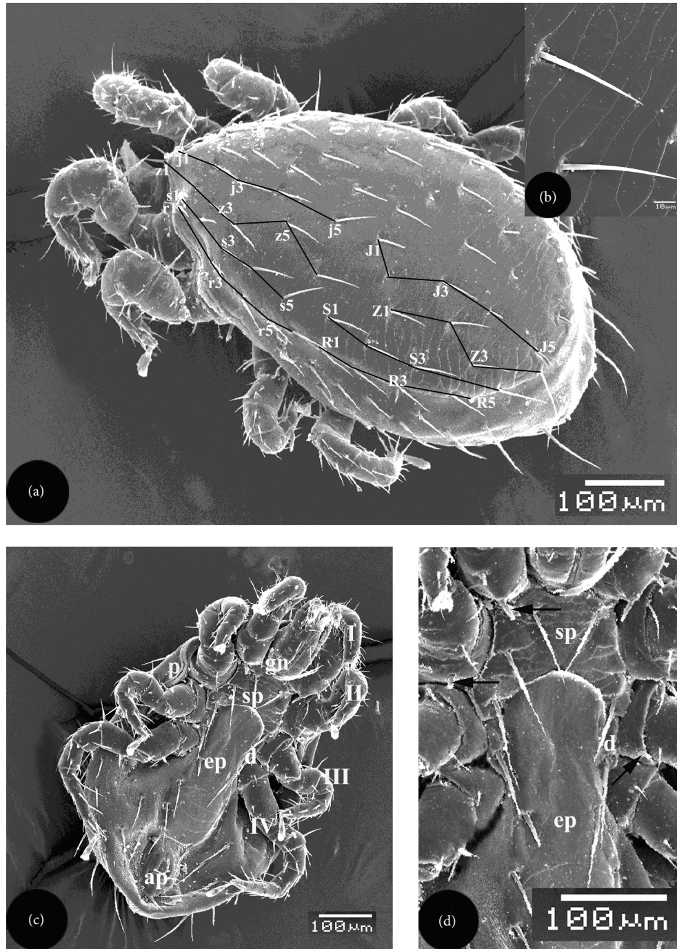
FIGURE 1: Scanning electron micrographs of dorsal and ventral surfaces of female Laelaps nuttalli . (a) Chaetotaxy of the dorsal shield showing distribution of 40 pairs of setae. Black lines connect setal sockets in each series which include j1-j5, z1-z6, s1-s5, r1-r6, J1-J5, Z1-Z4, S1-S4, and R1-R5. (b) Posterior region of dorsal shield showing long pointed setae and considerable striations. (c) Whole ventral side showing gnathosoma (gn), sternal plate (sp), epigynial plate (ep), endapodal plate (d), anal plate (ap), peritreme (p), and 4 pairs of legs (I-IV). (d) Sternal plate (sp) carrying 3 pairs of long pointed setae, epigynial plate (ep) carrying 4 pairs of pointed setae, endapodal plate (d) carrying 1 long pointed seta, and coxae of the first three legs carrying short stout posteriorly directed spurs (arrows).
