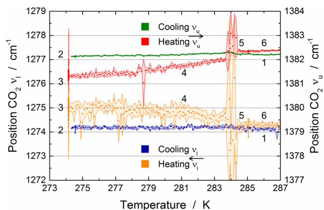
Figure 7. Positions of the upper ( \nu_{\text{u}} ) and lower ( \nu_{\text{l}} ) band of the CO 2 Fermi dyad during one measurement cycle.
