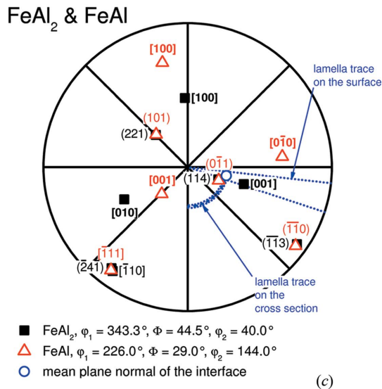
Figure 4 (a) Orientation mapping according to the inverse pole figure of the surface normal on a cross section of the arc-melted button (see insets; centre of the IPF of FeAl 2 corresponds to [001] FeAl 2 Chumak , standard triangle of FeAl encloses [100] FeAl , [110] FeAl and [111] FeAl ). Blue lines indicate minima and maxima of the lamella trace rotation with respect to the horizontal edge of the colony in the centre of the image. (b) An example of a SEM micrograph on a cross section prepared by FIB (secondary electron contrast, tilt-corrected). The blue dashed line indicates the mean of the lamella trace inclination with respect to the sample surface obtained from several cross sections. The standard deviation is highlighted by dotted lines. (c) Stereographic projection of the determined orientations of the colony in the centre of (a). Blue lines indicate rotation and inclination of the lamella traces according to (a) and (b). The complete set of stereographic projections for all colonies in (a) is provided as supporting information. For the pole projection of lattice planes, the normal vector of the planes is used.
